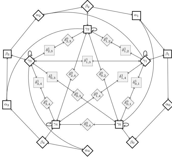
Figure 4: Game \mathfrak{D}_{\mathbb{S}}^4 of the SCC family.
